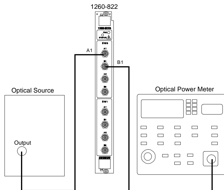
Figure C-4, Setup for Repeatability and Accuracy Procedure
