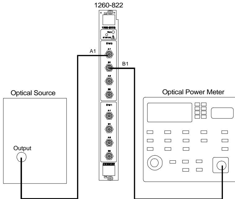
Figure C-1, Setup for Switch Disable Procedure
