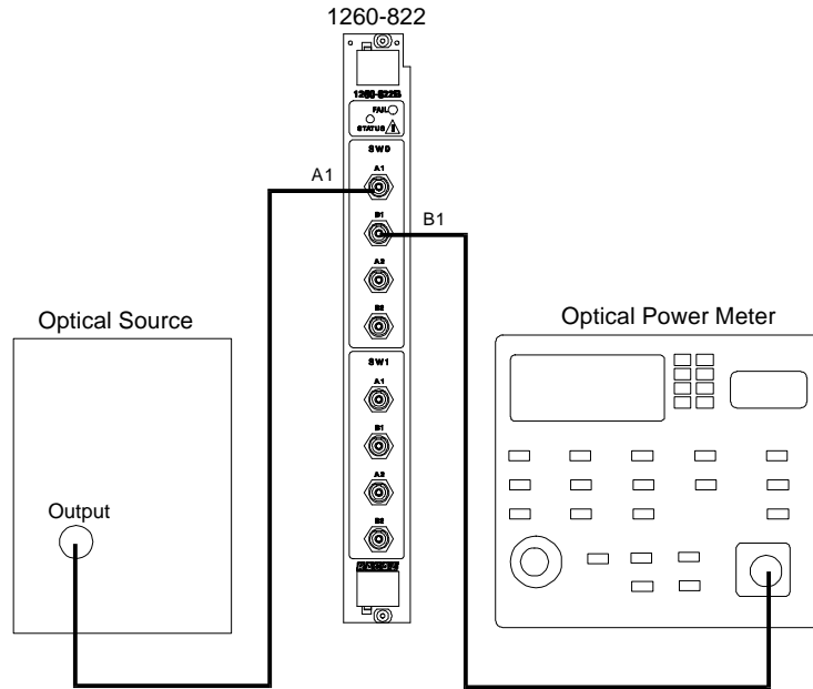
Figure C-3, Second setup for Insertion Procedure
