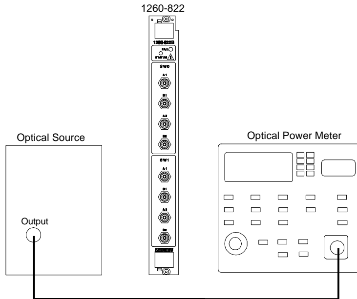
Figure C-2, First setup for Insertion Loss Procedure
