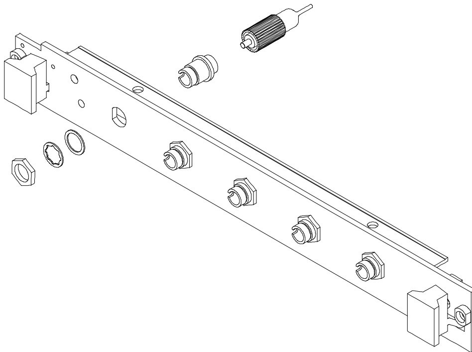
Figure B-1, Cleaning the Optical Connectors
